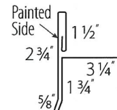
1 pc GABLE TRIM
