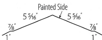
STARTER BASE / STANDING SEAM
