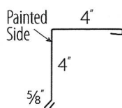
RAKE TRIM
