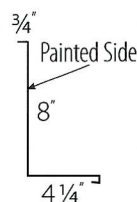
CHIMNEY FLASHING
