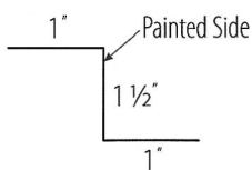
Z CLOSURE
