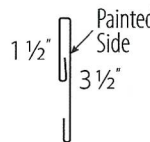
GABLE TRIM
