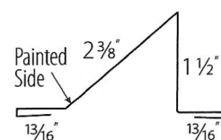
MRC SNOW GUARD
